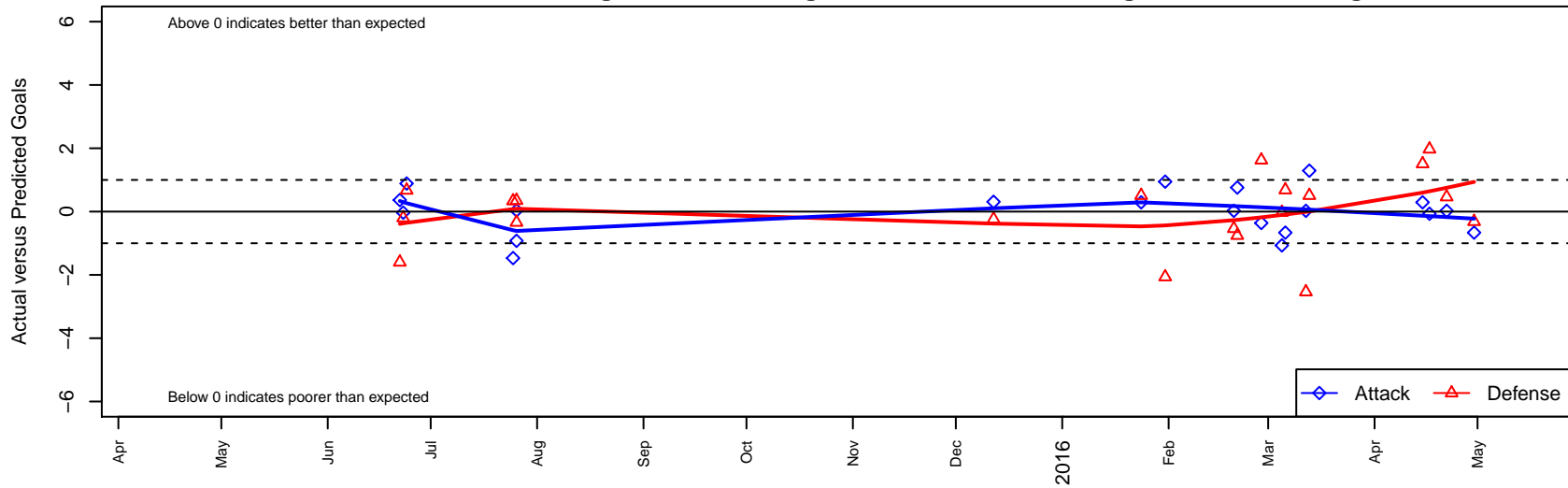
SSC Shadow A G97 Dots are actual minus expected GF (blue circles) and GA (red triangles). Blue line is smoothed change in attack strength. Red is smoothed change in defense strength.
